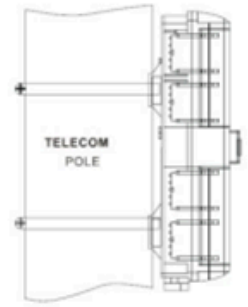
Pole ring installation
